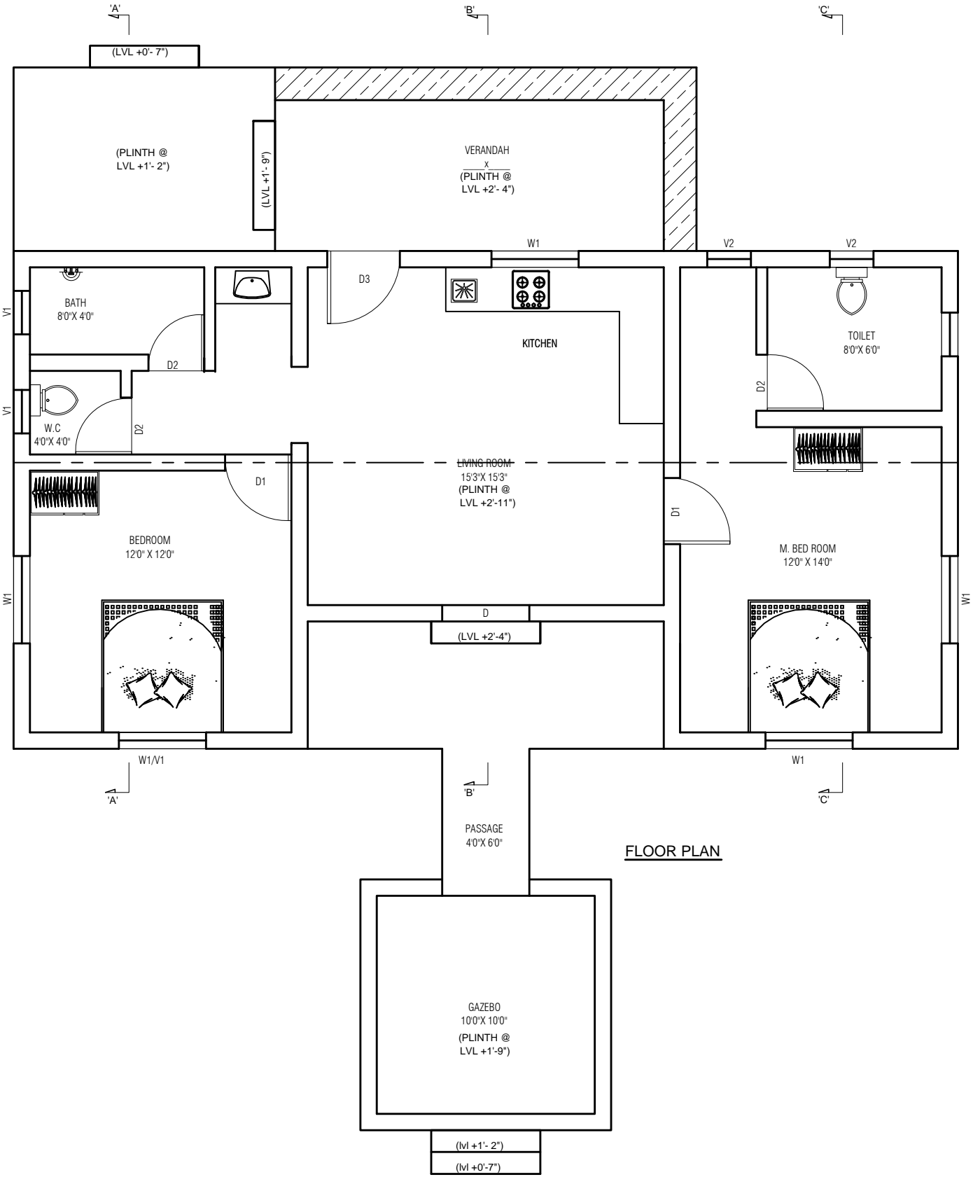
FLOOR PLAN
